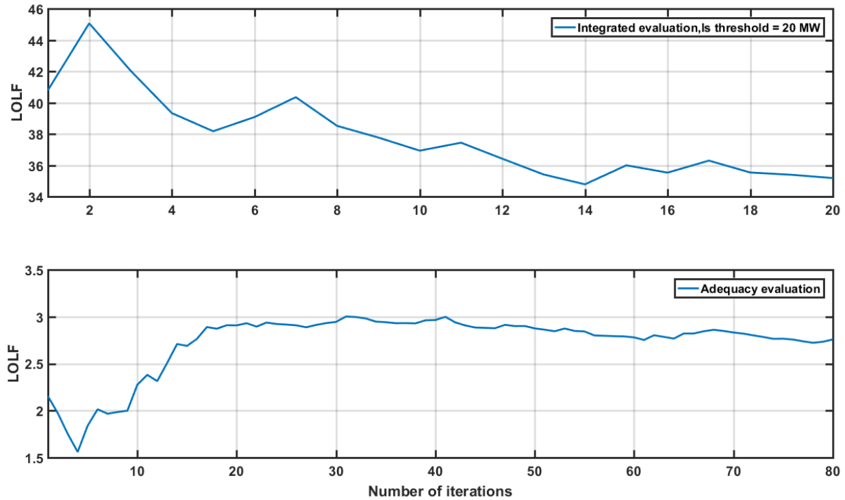
Figure 5.13 Convergence trajectory of LOLF comparison: adequacy Vs. adequacy and transient stability
