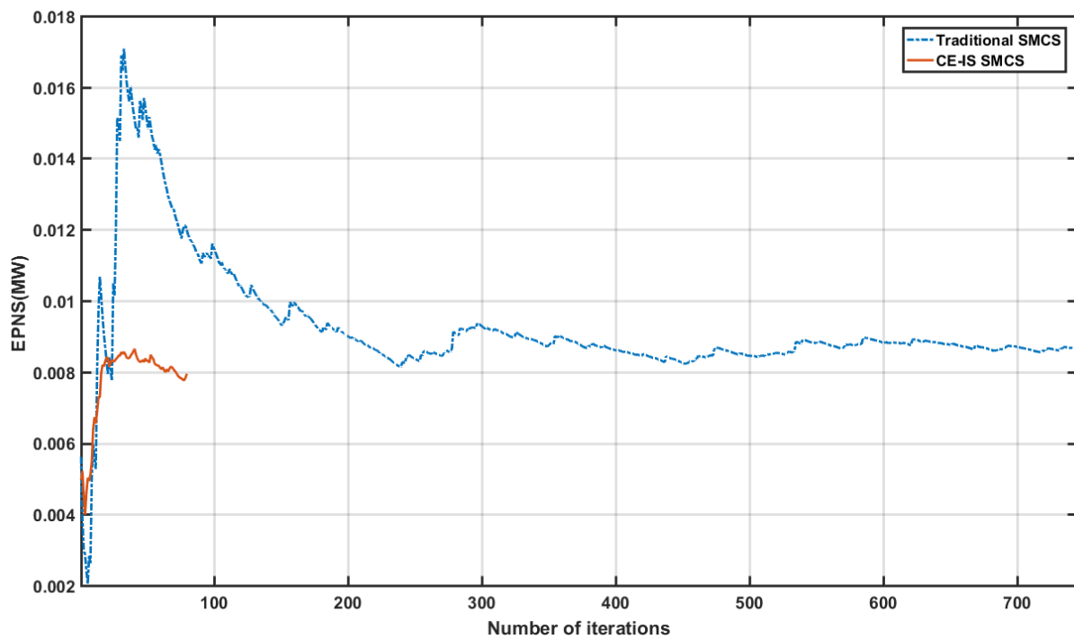
Figure 5.8 Convergence trajectory of EPNS from adequacy assessment based on CE-IS SMCS
