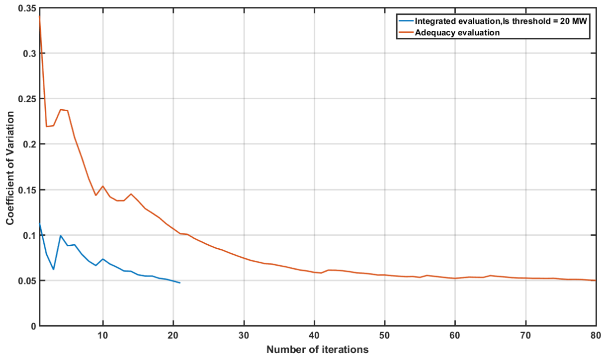
Figure 5.10 Convergence trajectory of COV comparison: adequacy Vs. adequacy and transient stability
