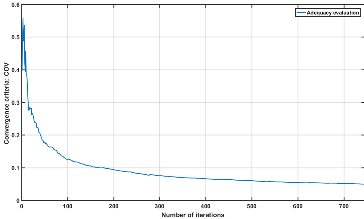
Figure 5.2 Convergence trajectory of COV from adequacy assessment based on SMCS
