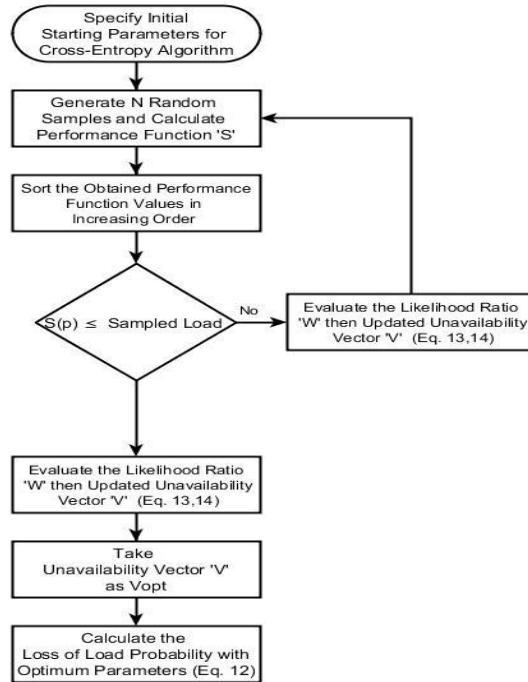
Figure 4.2: Flow Chart of Importance Sampling
