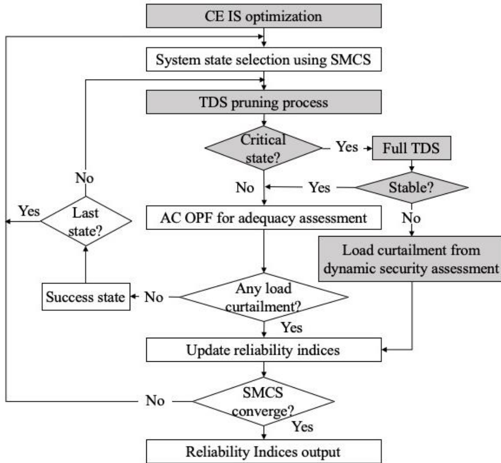
Figure 4.3 Reliability evaluation procedure with accelerating process
