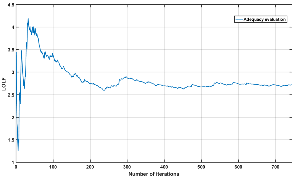
Figure 5.5 Convergence trajectory of LOLF from adequacy assessment based on SMCS
