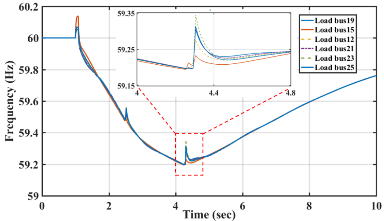
Figure 5.14 Load bus frequency under contingency
