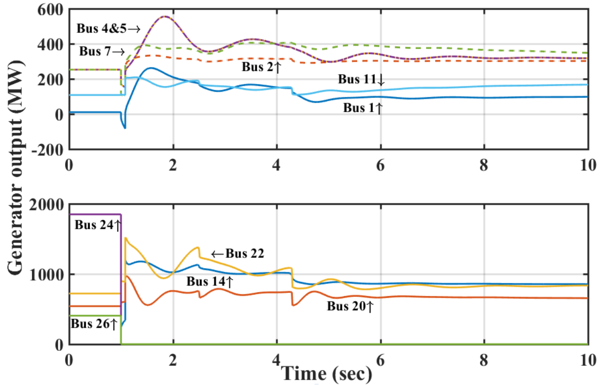
Figure 5.15 Generator output under contingency
