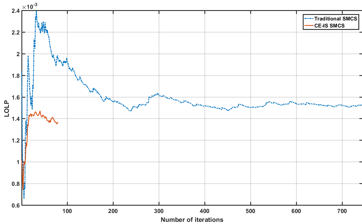
Figure 5.7 Convergence trajectory of LOLP from adequacy assessment based on CE-IS SMCS
