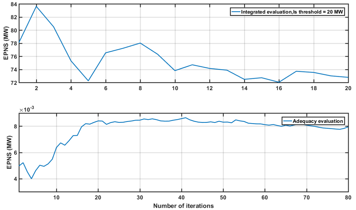
Figure 5.12 Convergence trajectory of EPNS comparison: adequacy Vs. adequacy and transient stability
