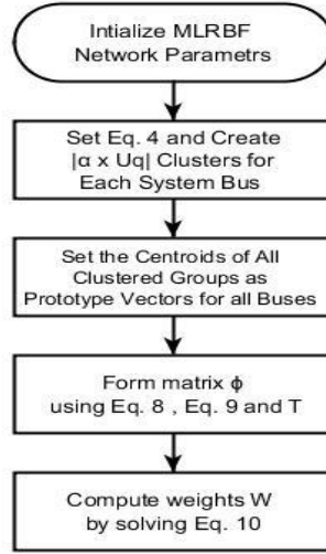
Figure 4.1: Flowchart Describing Training Phase of MLRBF
