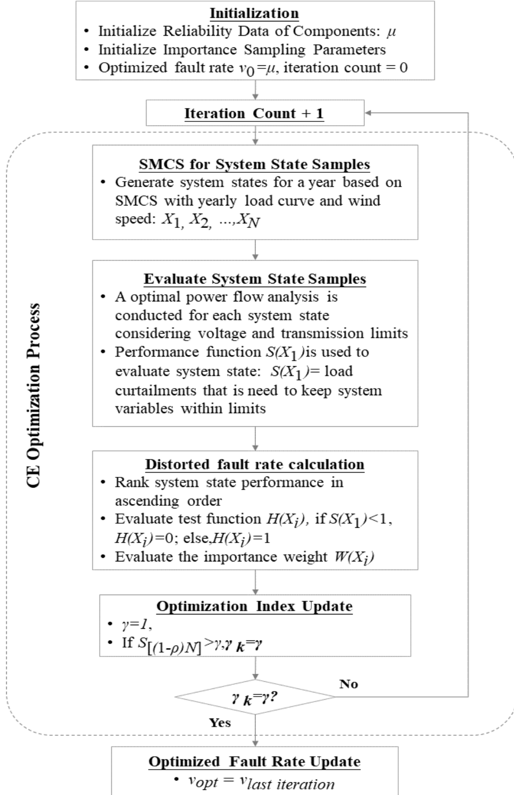
Figure 4.2 CE-IS optimization procedure
