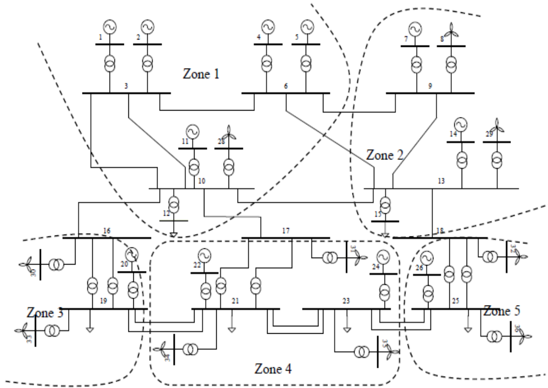
Figure 5.1 Synthetic test system
