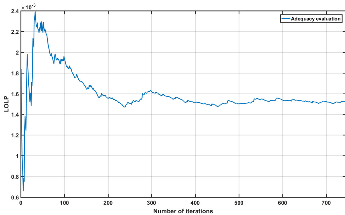
Figure 5.3 Convergence trajectory of LOLP from adequacy assessment based on SMCS
