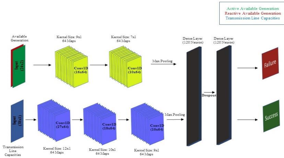
Figure 5.1: Overall Diagram of Proposed CNN Structure
