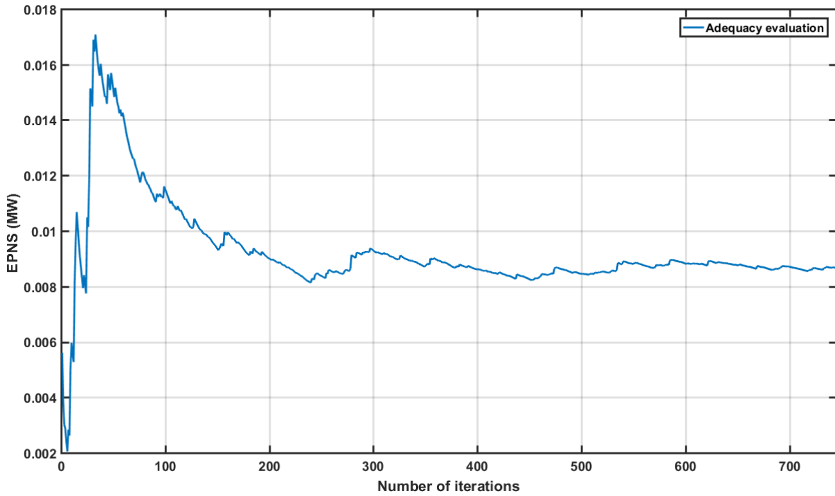
Figure 5.4 Convergence trajectory of EPNS from adequacy assessment based on SMCS
