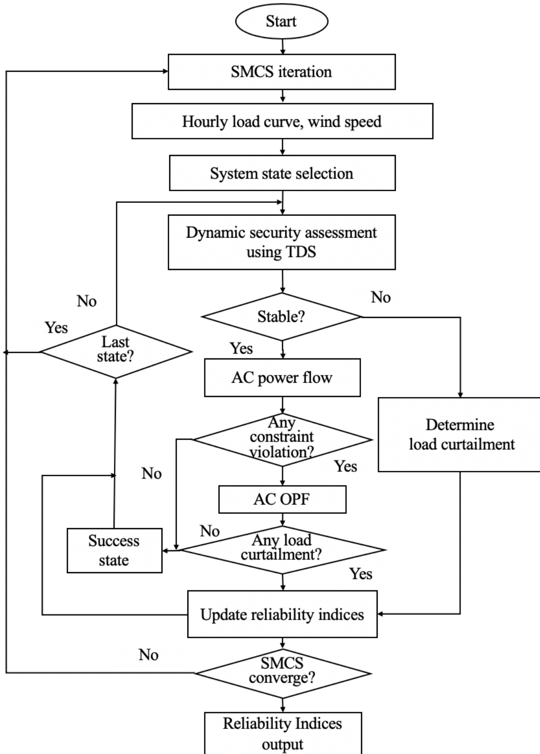
Figure 4.1 Flow chart for reliability evaluation with adequacy and transient stability integrated
