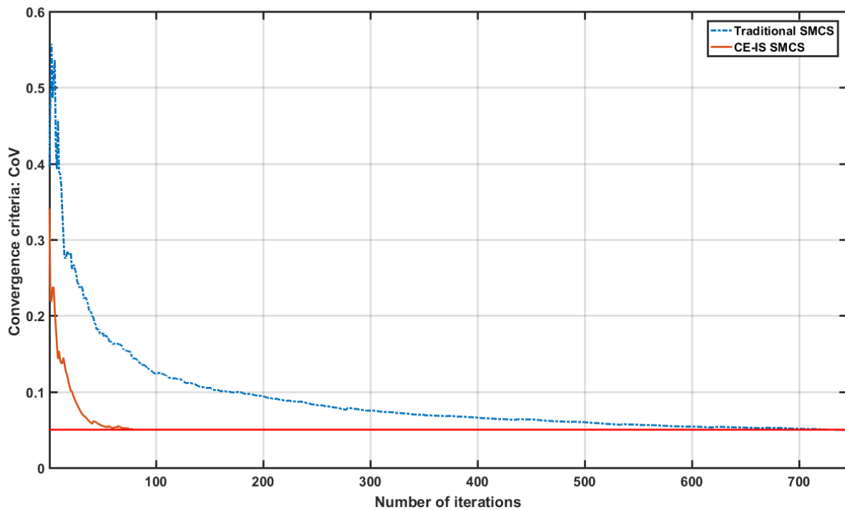
Figure 5.6 Convergence trajectory of COV from adequacy assessment based on CE-IS SMCS
