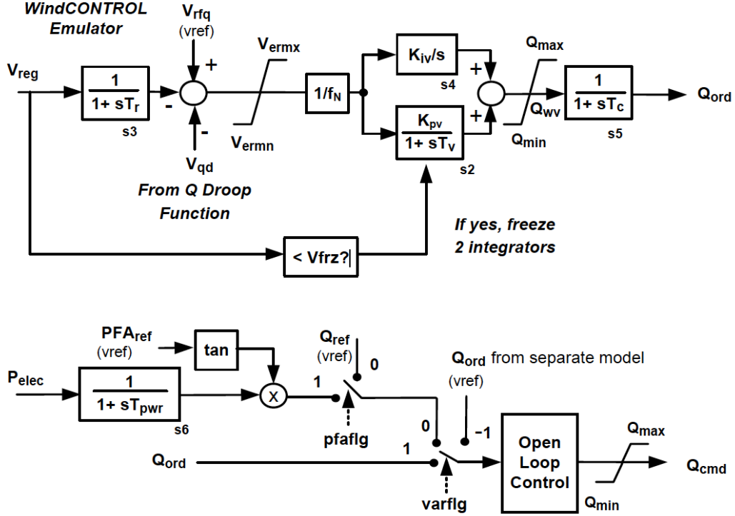
Figure 3.7 Reactive power control model
