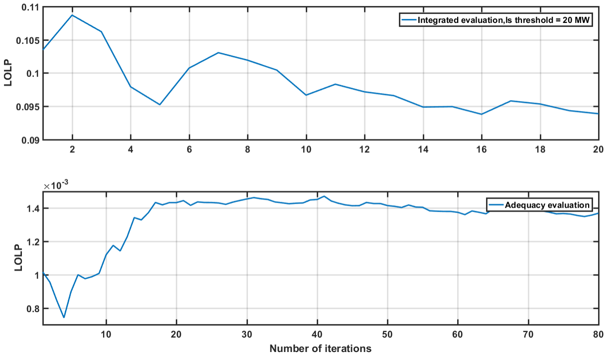
Figure 5.11 Convergence trajectory of LOLP comparison: adequacy Vs. adequacy and transient stability
