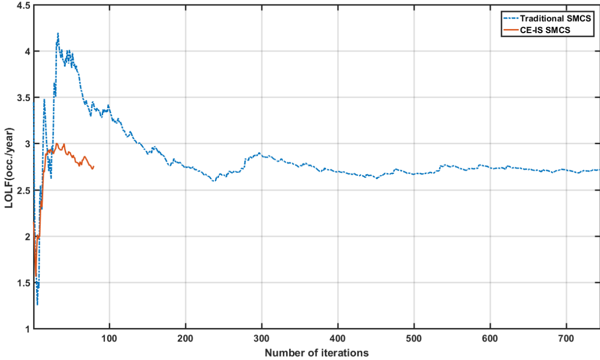
Figure 5.9 Convergence trajectory of LOLF from adequacy assessment based on CE-IS SMCS
