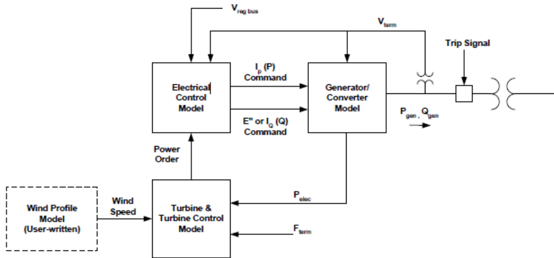
Figure 3.5 GE WTG Dynamic Model Connectivity
