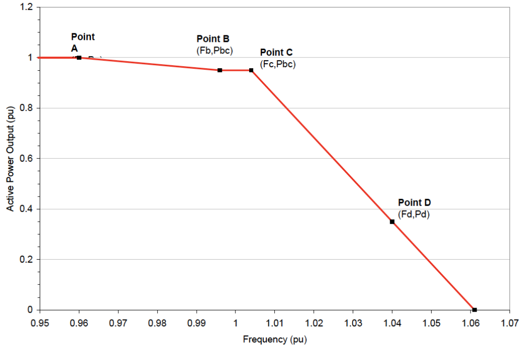
Figure 3.6 Frequency response curve
