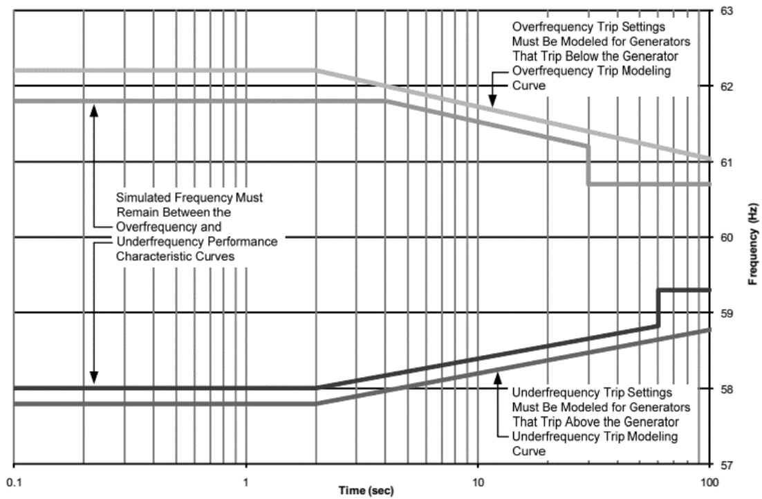
Figure 3.8 Design performance and modelling curves for over and under frequency generator trip [34]
