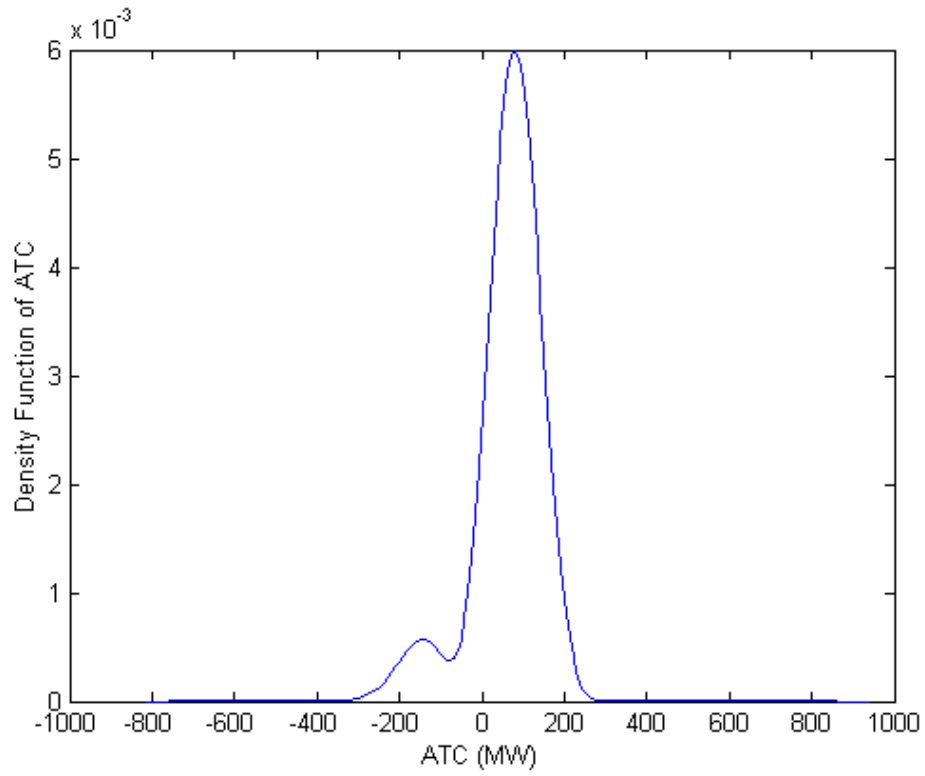
Figure B.7 PDF of the ATC in line 1-5 in Example14S1-15 with line 1-5 in service
