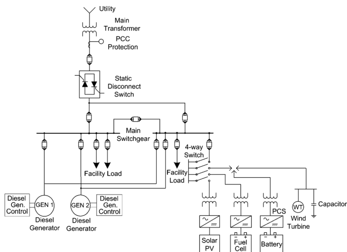
Fig. 1. Santa Rita Jail Microgrid Single Line Diagram.
