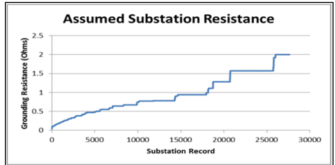
Figure 2: Sorted Substation Grounding Resistance
