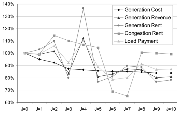
Fig. 9. Value propagations with J for expensive generators sensitivity.
