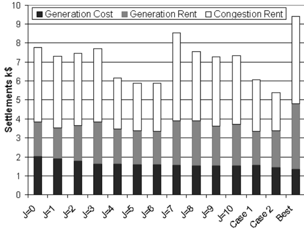
Fig. 2. Load payments and wealth transfers.
