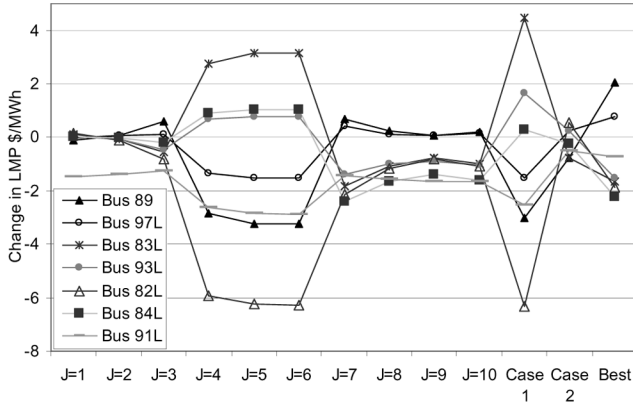
Fig. 5. Change in LMP values.
