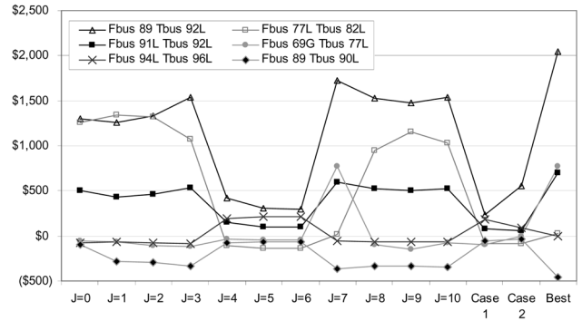
Fig. 6. Congestion rent fluctuations.
