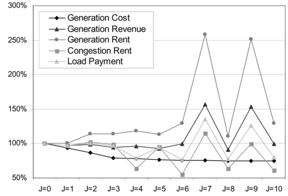
Fig. 8. Value propagations with J for bus angle sensitivity.
