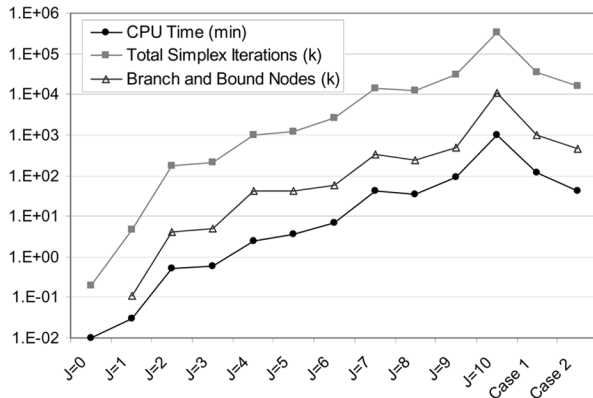
Fig. 7. Computational statistics on computation time, simplex iterations, and branch and bound nodes.
