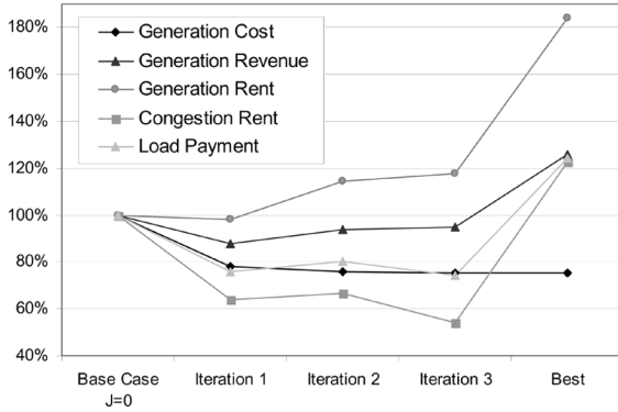
Fig. 11. Value propagations for base case and heuristic approach sensitivity study.
