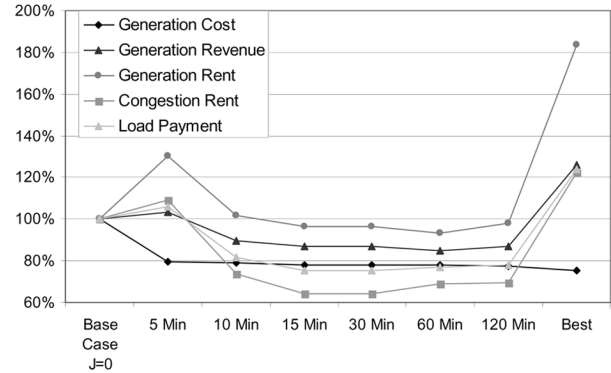
Fig. 10. Value propagations for various stopping times compared to original base case J = 0 for stopping time sensitivity.
