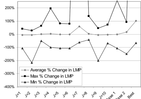
Fig. 3. Average, max, and min percent change in LMP.
