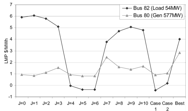
Fig. 4. Dispatched generator and load bus with largest LMP variance. The buses with the largest variance (mean square deviations) in LMP for these two categories are displayed.
