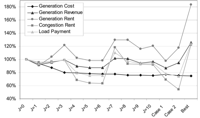
Fig. 1. Generation cost, generation revenue, generation rent, congestion rent, and load payment for various solutions.
