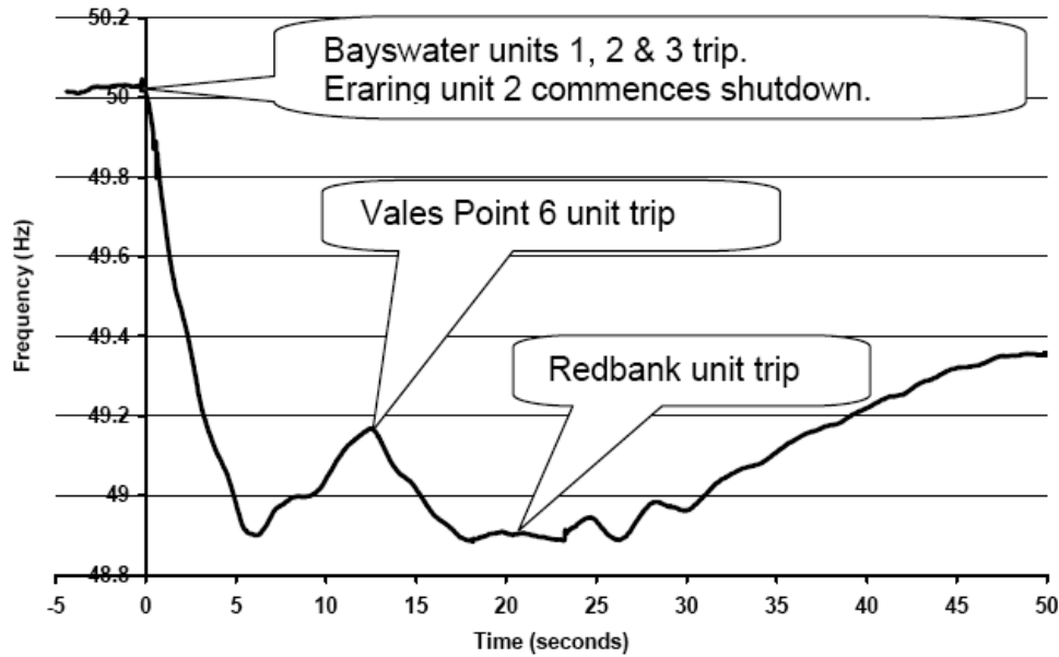
Figure 1. Australian Generation-Loss Experience: System Frequency Over Time (source [4])
