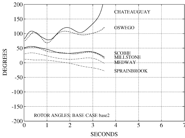
Fig. 6. Base case for Selkirk fault.
