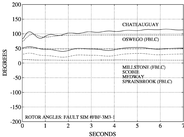
Fig. 8. Rotor angle response with advanced FBLC controller.
