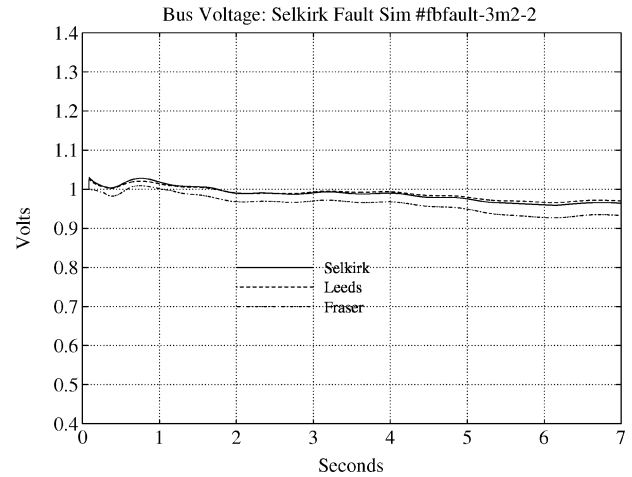
Fig. 9. Voltage response with advanced FBLC controller.
