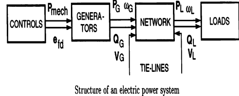
Fig. 4. Structure of an electric power system.
