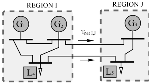
Fig. 2. An interconnected 5-bus power system.
