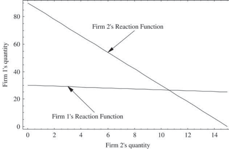
Figure 2. Reaction functions for case B (no transmission constraints).
