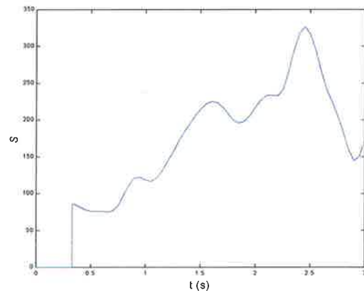
Figure 8: The plot of S vs. time for t_{cl} = 0.28 s.
