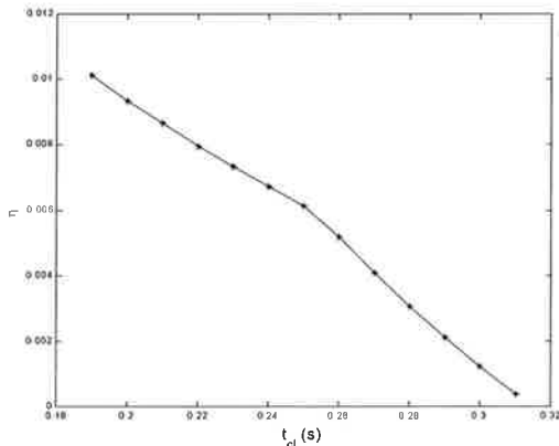
Figure 10: Estimate of t_{cr} for 50-machine system.
