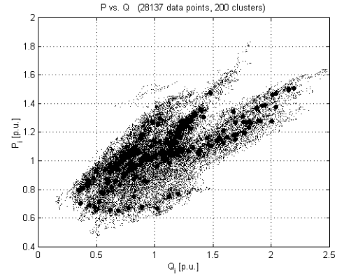
Fig. 10. The data and cluster center points (projection onto the P-Q plane).
