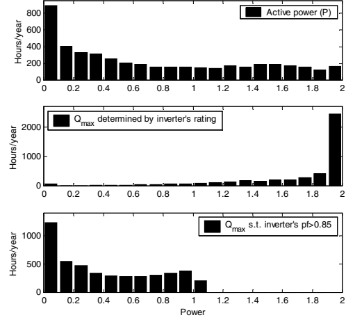
Fig. 6. Histograms of annual inverter active energy production and corresponding reactive production, limited by Q_{max} and Q_{lim} .
