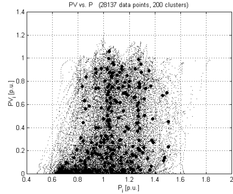
Fig. 9. The data and cluster center points (projection onto the PV-P plane).
