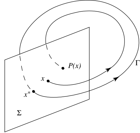
Figure 1: Poincaré map.
