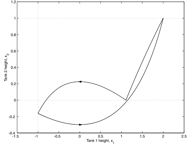
Figure 4: Limit cycle.
