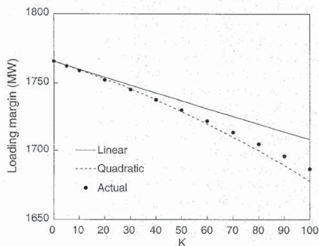
Figure 6. Effect of composition of load model
