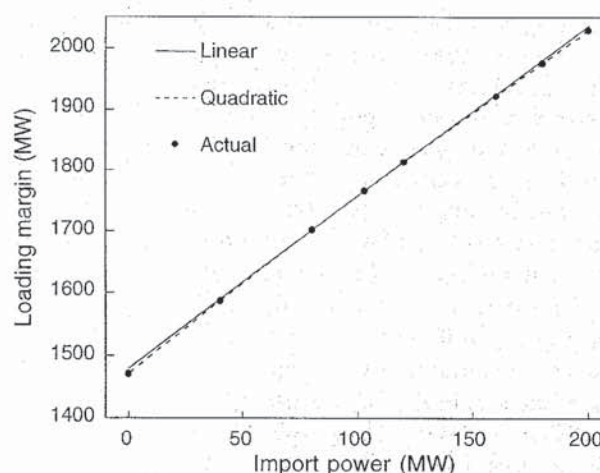
Figure 5. Effect of import into critical area
