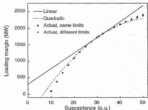
Figure C1. Effect of susceptance of line 9-10
